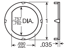
Pronged Washer 253F2680002G Pin tumbler for single flat
